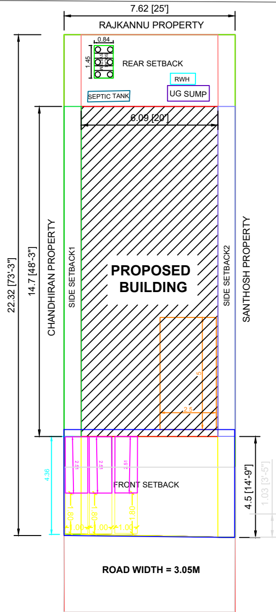
LOCATION PLAN NOT TO SCALE
