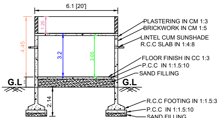
SECTION PLAN
