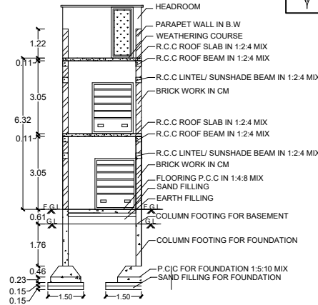
SECTION ON-AA
