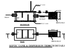
SEPTIC TANK & DISPERSION TRENCH DETAILS
