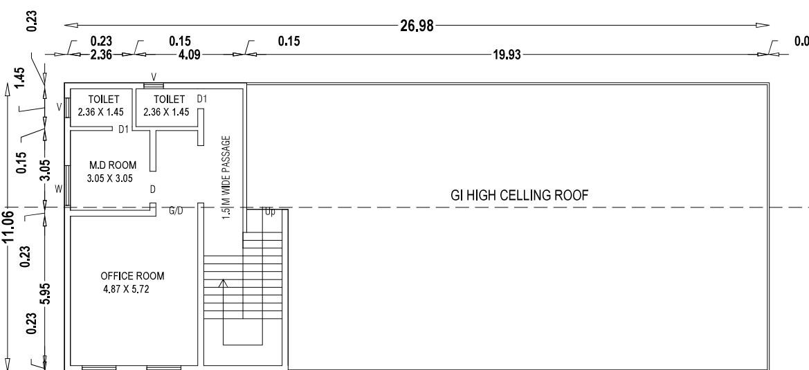
MEZZANINE FLOOR PLAN
