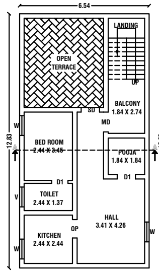
RESIDENTIAL SECOND FLOOR PLAN
