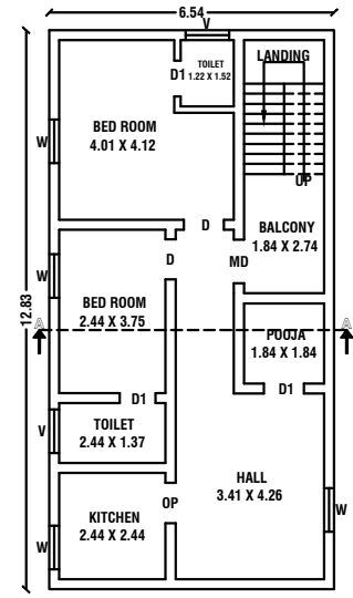
RESIDENTIAL FIRST FLOOR PLAN
