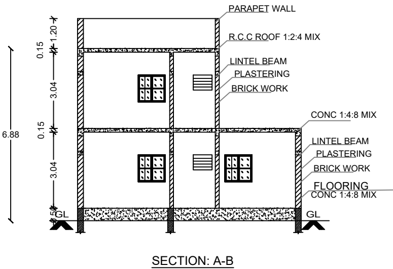
SECTION: A-B
