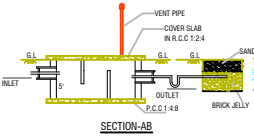
SECTION-AB
