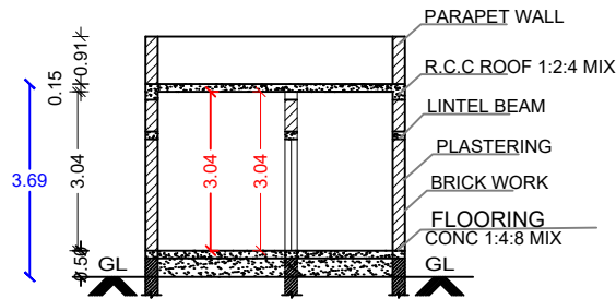
SECTION: A-B
