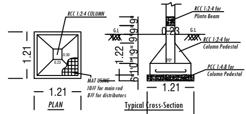
FOOTING DETAILS
