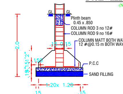
FOUNDATION DETAIL
