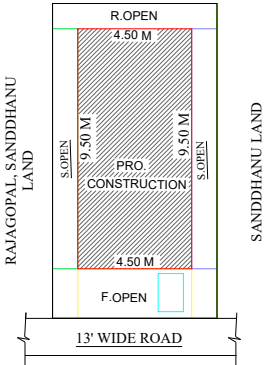
SITE PLAN
