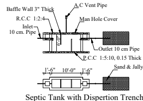
Septic Tank with Dispersion Trench
