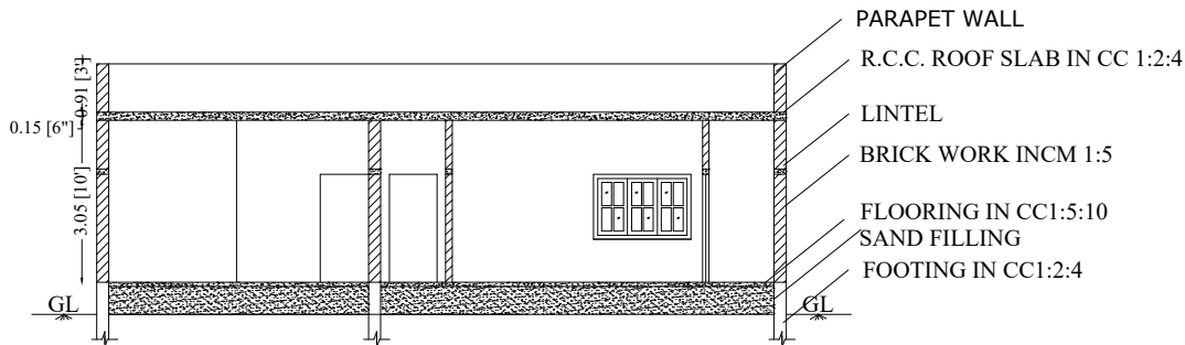
SECTION ON "AA"
