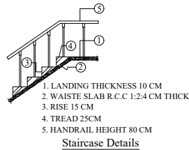
Staircase Details
