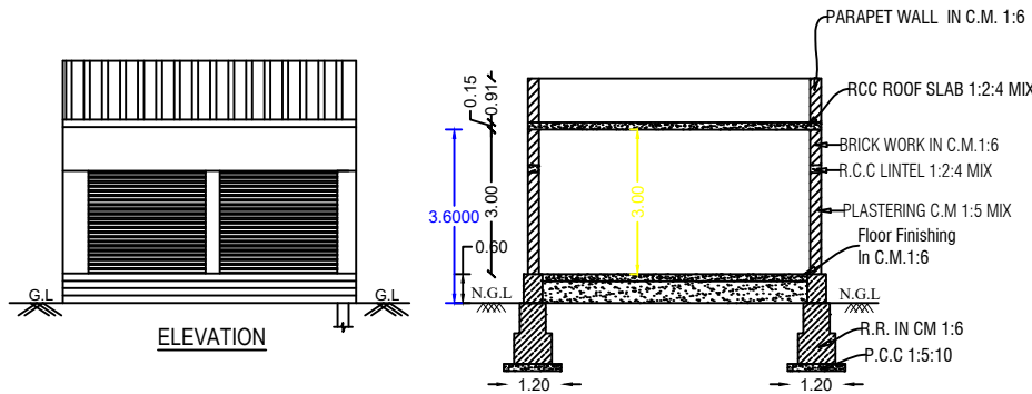
Section On-"AB"
