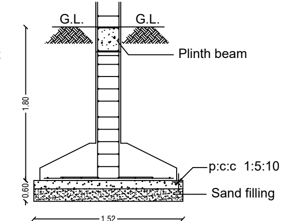
FOUNDATION DETAILS
