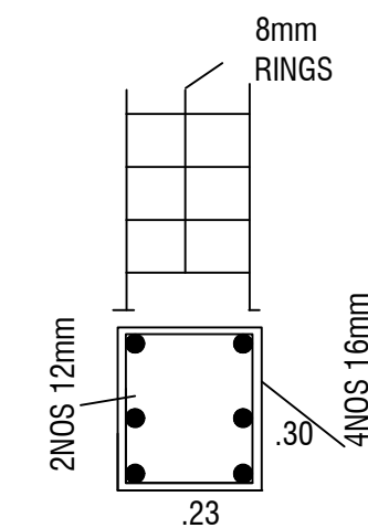
COLUMN DETAILS
