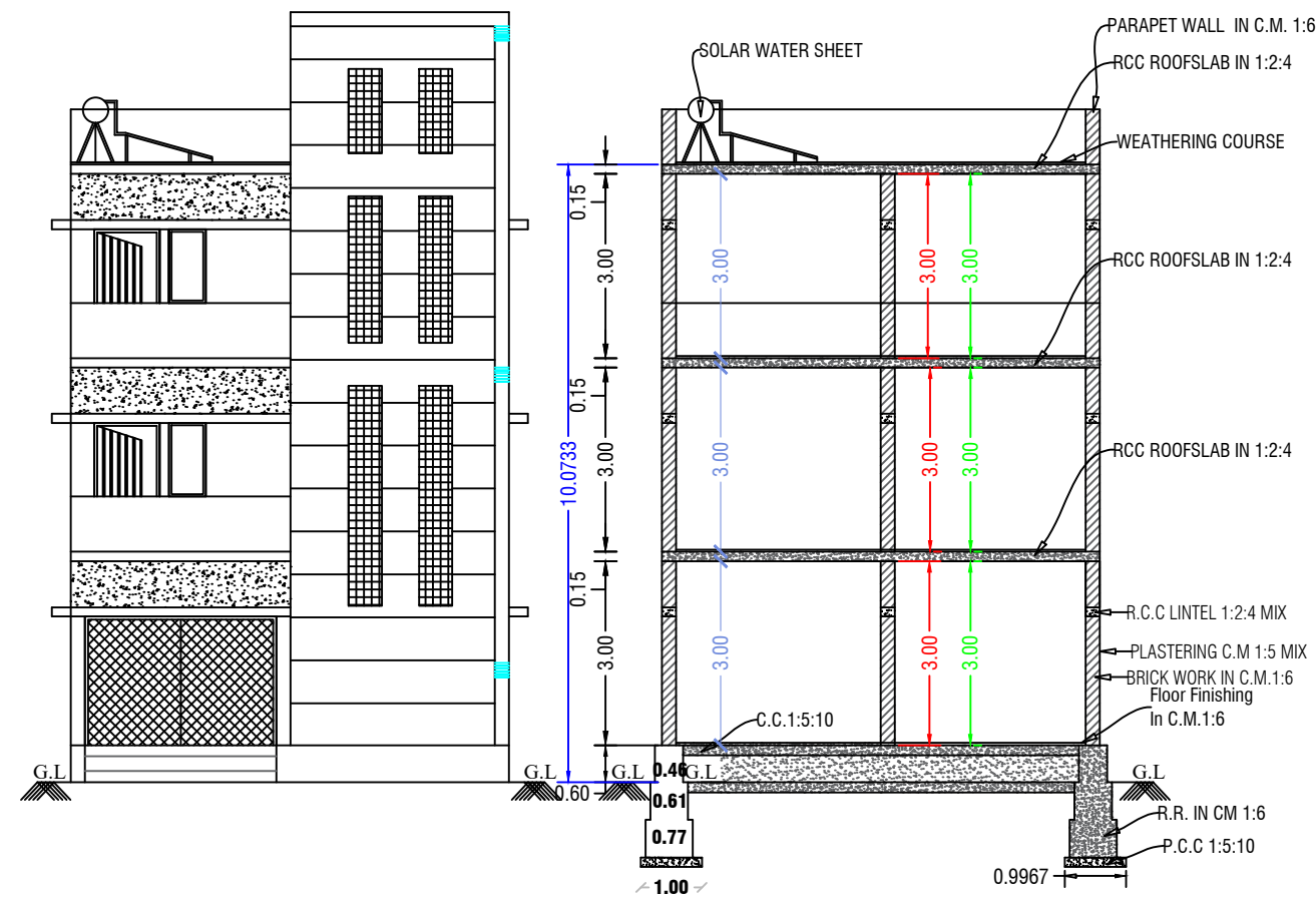
Section On-'AB'
