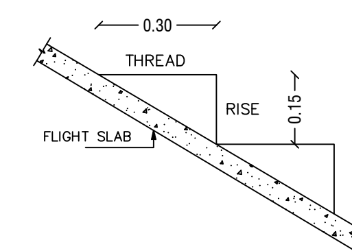
STAIRCASE DETAILS
