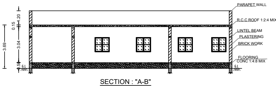
SECTION : "A-B"
