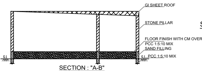
SECTION : "A-B"
