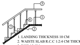
Staircase Details
