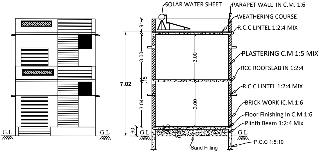
ELEVATION PLAN
