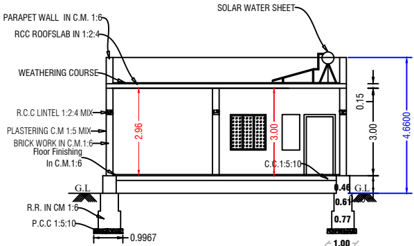
SECTION
