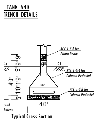
FOOTING DETAILS
