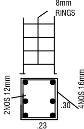
COLUMN DETAILS
