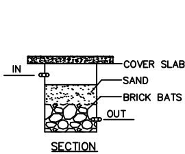
RAINWATER HARVEST
