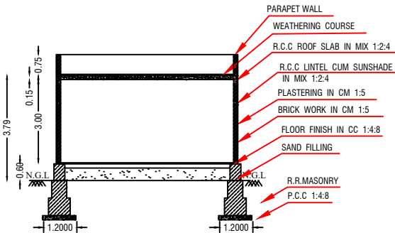
SECTION ON-'AB'
