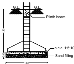
FOUNDATION DETAILS
