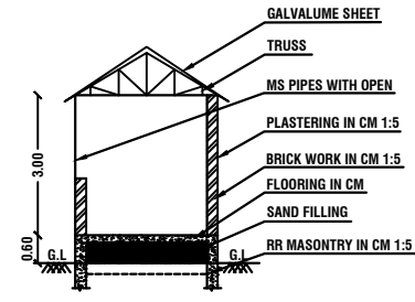
SECTION ON - AB
