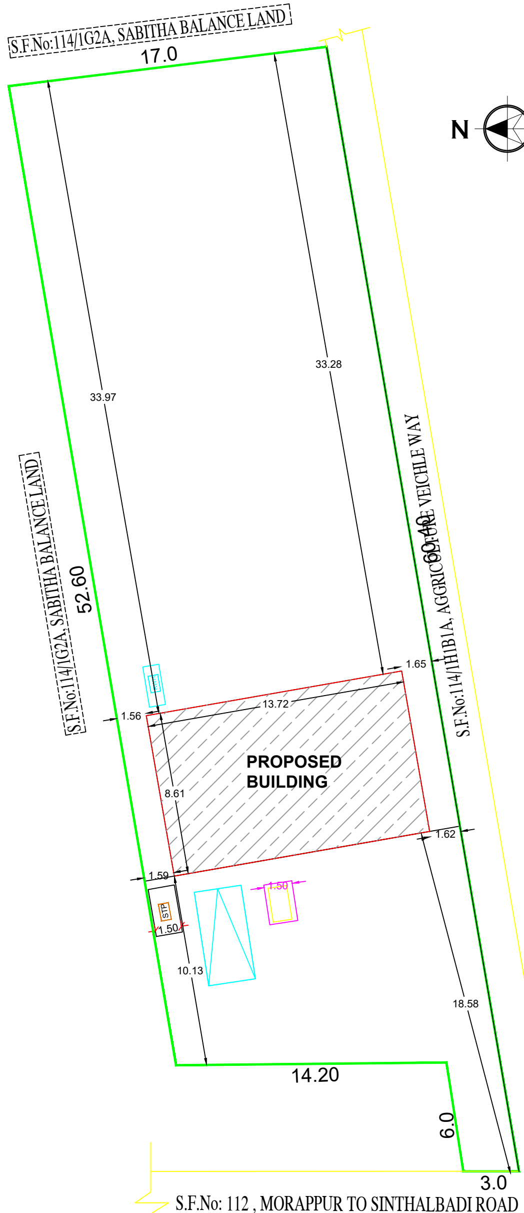
SITE PLAN
