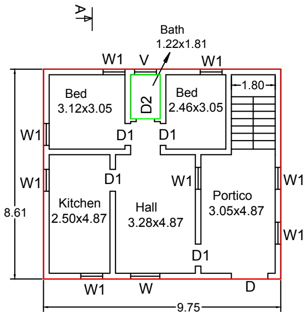
PLAN - Ground Floor
