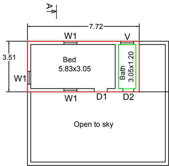
PLAN - First Floor
