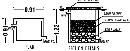
RAINWATER HARVESTING SYSTEM
