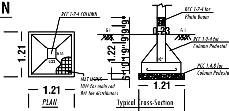
FOOTING DETAILS
