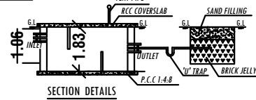
SECTION DETAILS
