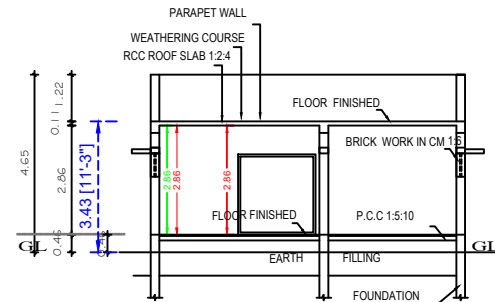
SECTION "A-B"
