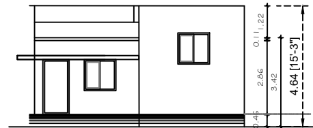
FRONT ELEVATION.
