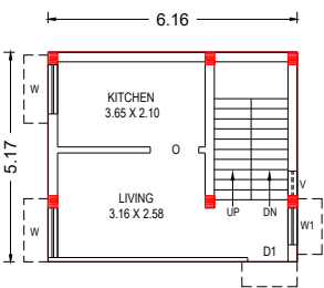
PRO. GROUND FLOOR PLAN.
