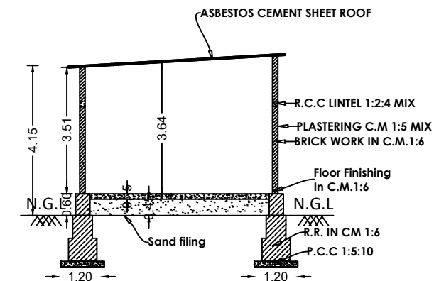
Section on-"AB"
