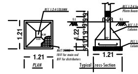
FOOTING DETAILS
