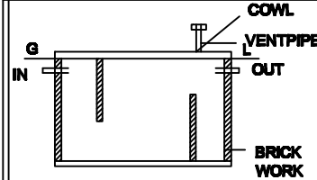
SECTION ON -XY
