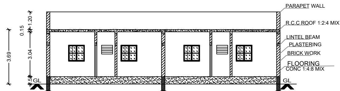
SECTION: A-B
