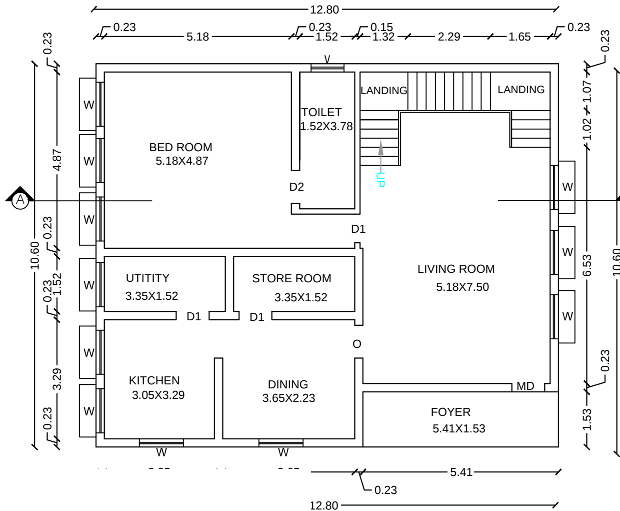
ND FLOOR PLAN
