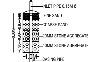
DETAILS OF RAIN WATER HARVESTING STRUCTURES SCALE- 1:20
