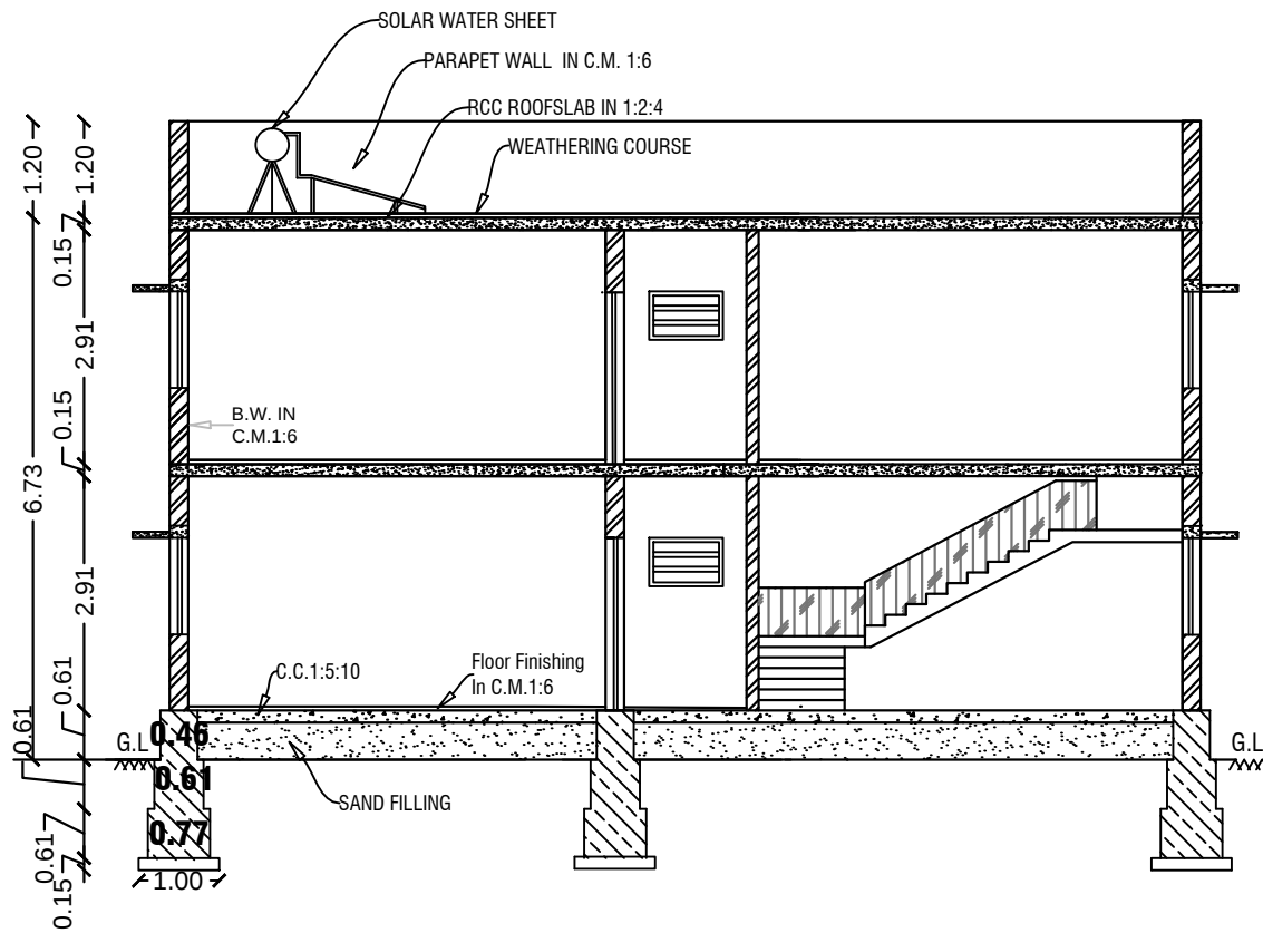
SECTION -AA
