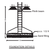
FOUNDATION DETAILS
