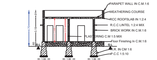
SECTION ON-'AB'
