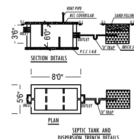
SEPTIC TANK AND DISPERSION TRENCH DETAILS
