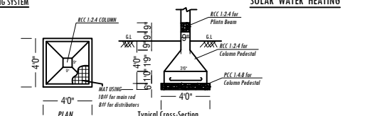
FOOTING DETAILS
