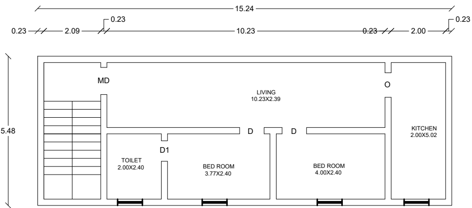
FIRST FLOOR
