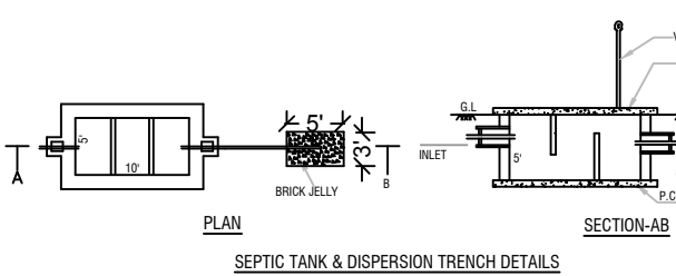
SEPTIC TANK & DISPERSION TRENCH DETAILS SCALE- 1:100
