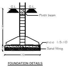
FOUNDATION DETAILS
