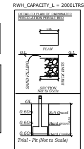
DETAILED PLAN OF RAINWATER PERCOLATION BED
