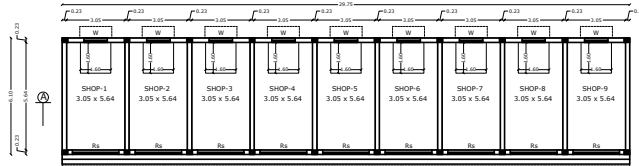
GROUND FLOOR PLAN
