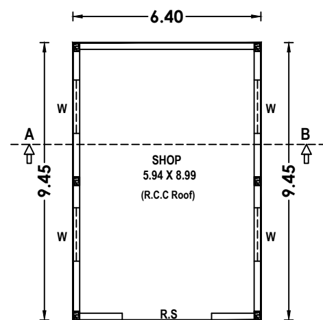
Ground Floor Commercial Plan
