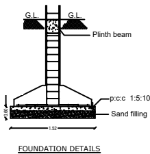
FOUNDATION DETAILS
