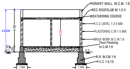
SECTION ON-'AB'
