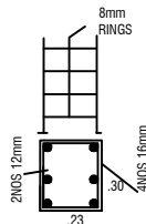
COLUMN DETAILS
