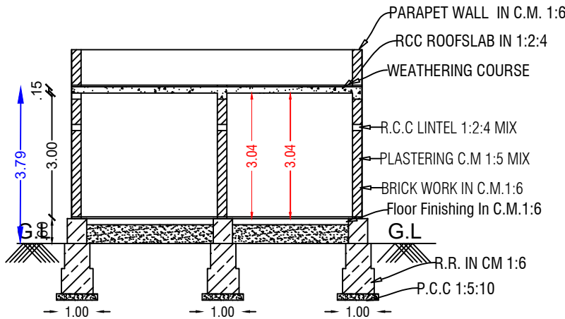
SECTION ON-"AB"
