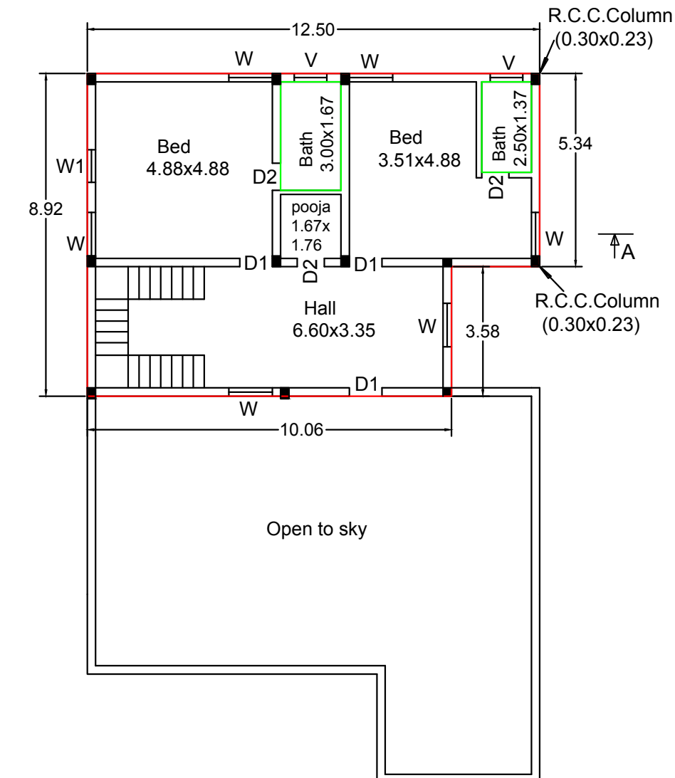
PLAN - FIRST FLOOR
