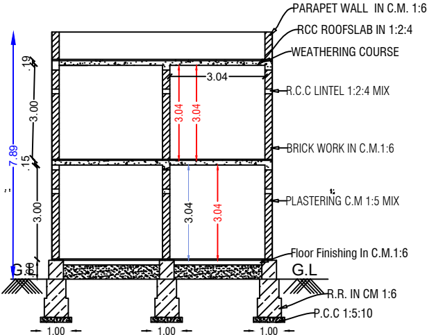
BLOCK 1 SECTION ON-"AB"
