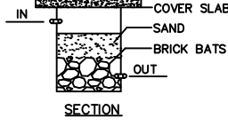
RAINWATER HARVEST
