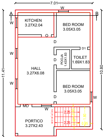
BLOCK 1 GROUND FLOOR PLAN
