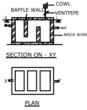
SEPTICTANK DETAILS
