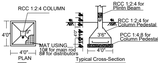
FOOTING DETAILS
