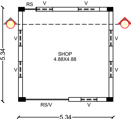
GROUND FLOORPLAN
