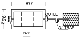
SEPTIC TANK AND SPERSION TRENCH DETAILS
