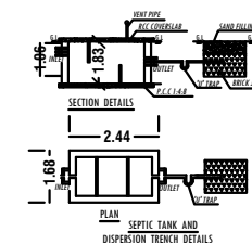
SEPTIC TANK AND DISPERSION TRENCH DETAILS
