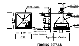
FOOTING DETAILS
