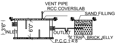
SECTION DETAILS
