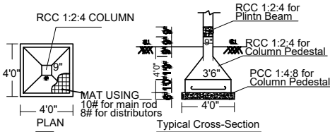
FOOTING DETAILS
