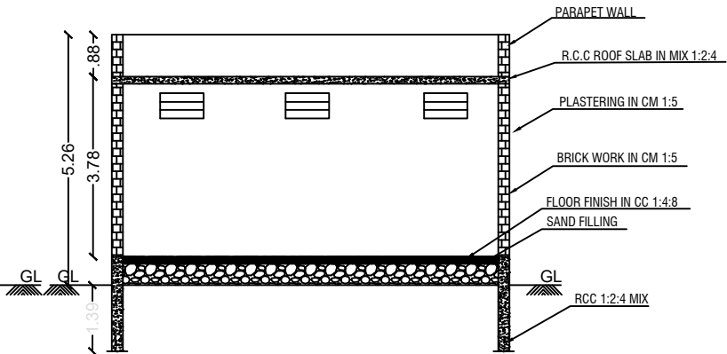
SECTION ON "MA"
