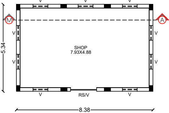
GROUND FLOORPLAN
