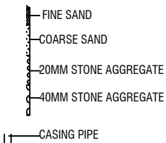
DETAILS OF RAIN WATER HARVESTING STRUCTURES
