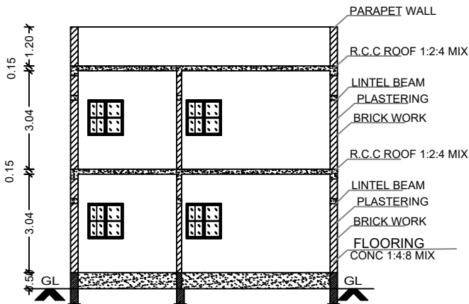
SECTION: A-B
