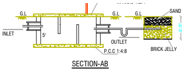
DETAILS OF RAIN WATER HARVESTING STRUCTURES
