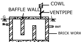
SECTION ON - XY
