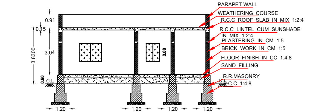
SECTION ON-"AB"
