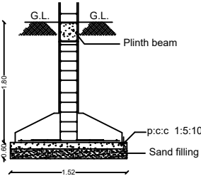
FOUNDATION DETAILS
