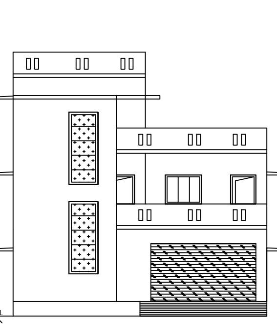
FRONT ELEVATION
