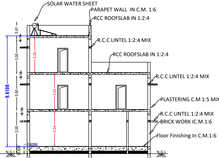
CROSS SECTION ON-"AB"
