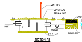
SECTION-AB
