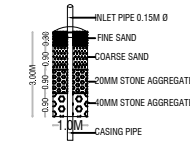
DETAILS OF RAIN WATER HARVESTING STRUCTURES
