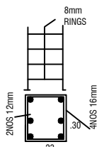
COLUMN DETAILS
