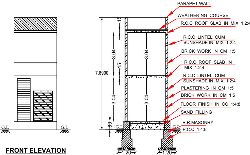
SECTION ON-"AB"
