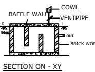
SEPTICTANK DETAILS
